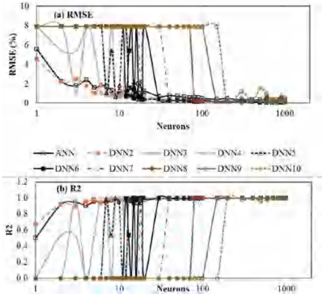
Figure 5. Optimisation of the number of the neurons per hidden layer when training the neural networks models.
