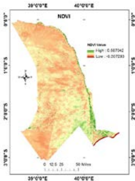
Figure 3.2: NDVI map
